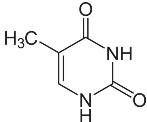
Thymin
